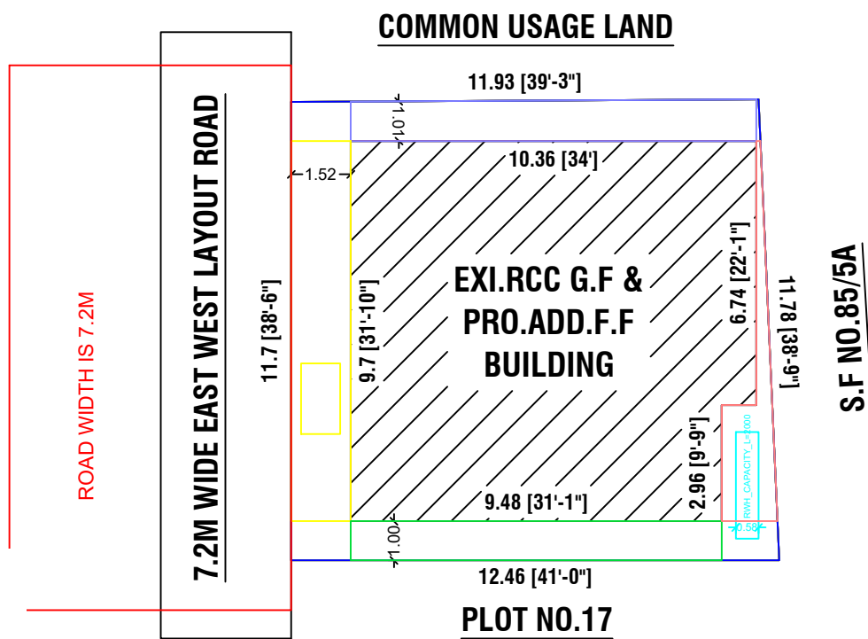
SITE PLAN
