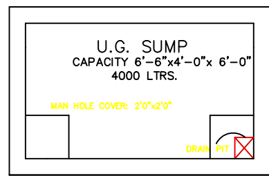
SUMP DETAIL
