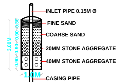
DETAILS OF RAIN WATER HARVESTING STRUCTURES
