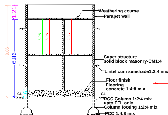
SECTION ELEVATION
