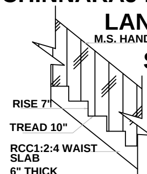
STAIRCASE DETAILS
