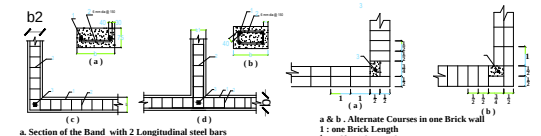
Figure - 2 : Reinforcement and Bending Details of Seismic Bands.
