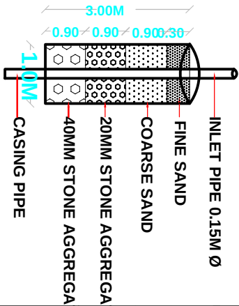
DETAILS OF RAIN WATER
