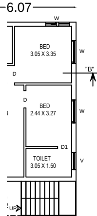
F PLAN
