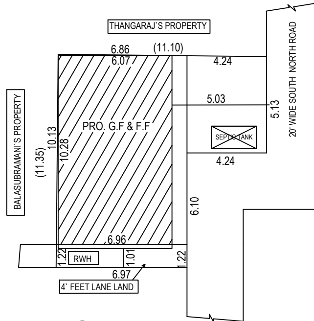
SITE PLAN
