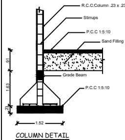
COLUMN DETAIL
