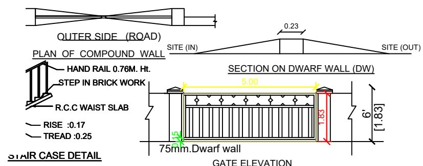
COMPOUND WALL DETAIL
