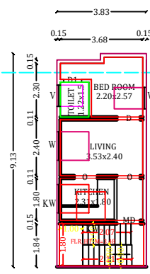
PRO.F.FLOOR PLAN
