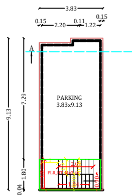
PRO.STILT FLOOR PLAN
