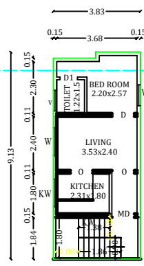
PRO.T.FLOOR PLAN
