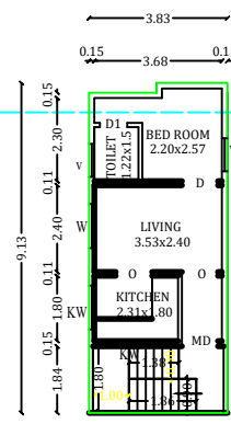
PRO.S.FLOOR PLAN
