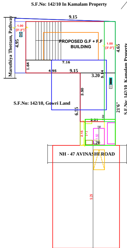
SITE PLAN
