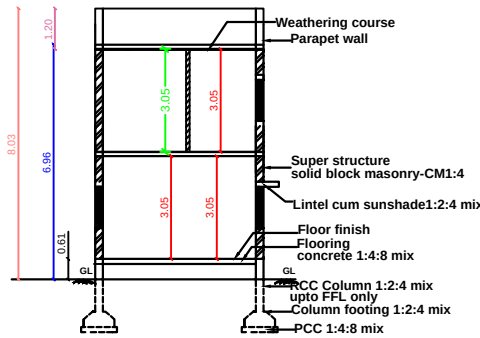
SECTION ELEVATION-AA
