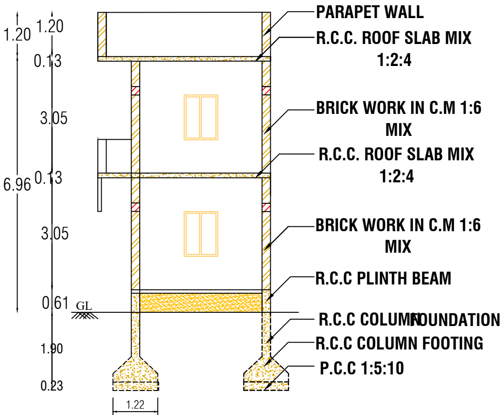
CROSS SECTION AT A-A
