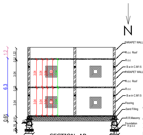
SECTION AB
