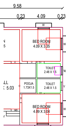
PROPOSED ADDITIONAL ST FLOOR PLAN
