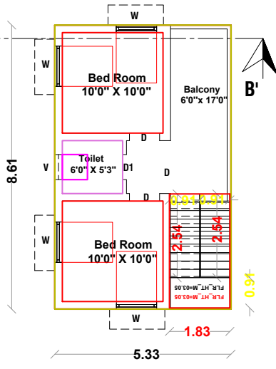
PROPOSED F.F PLAN [ Block 2 ]
