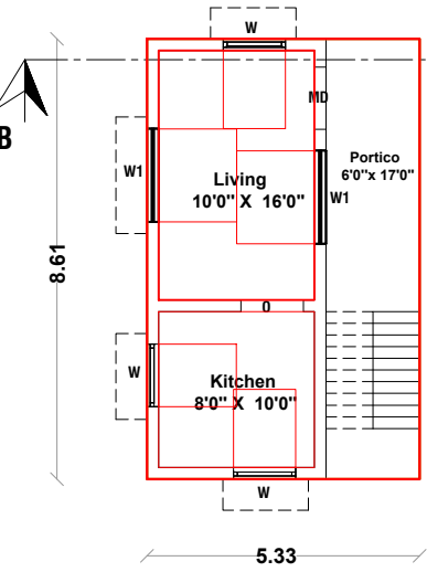
PROPOSED G.F PLAN [ Block 2 ]
