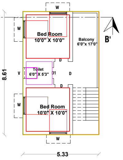
PROPOSED F.F PLAN [ Block 1 ]
