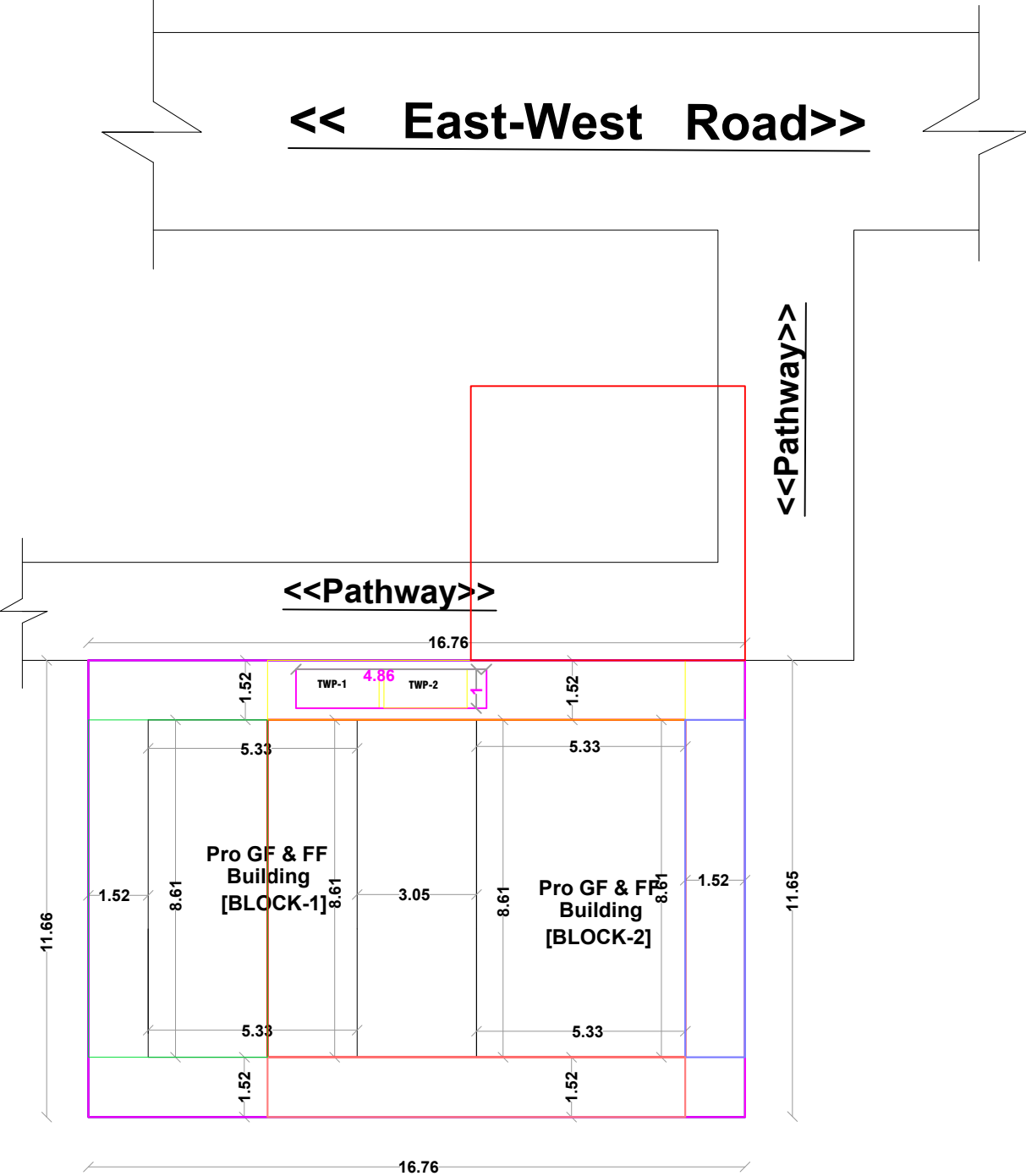
SITE PLAN
