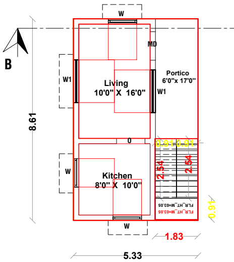
PROPOSED G.F PLAN [ Block 1 ]
