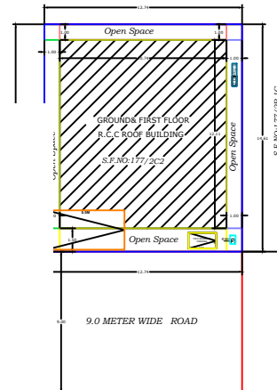
SUPER IMPOSED SITE PLAN
