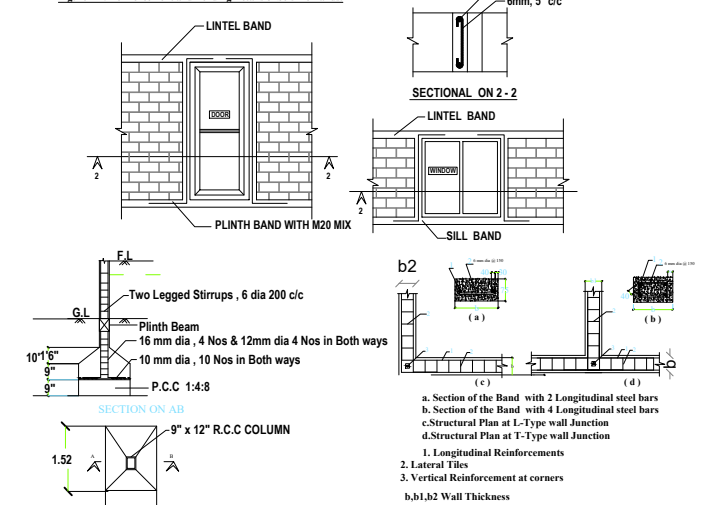
Figure - 2 : Reinforcement and Bending Details of Seismic Bands.
