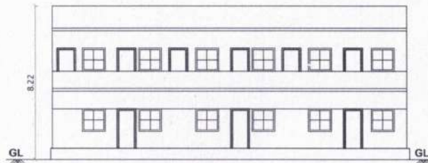
SOUTH SIDE ELEVATION
