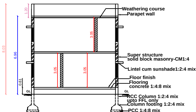
SECTION ELEVATION
