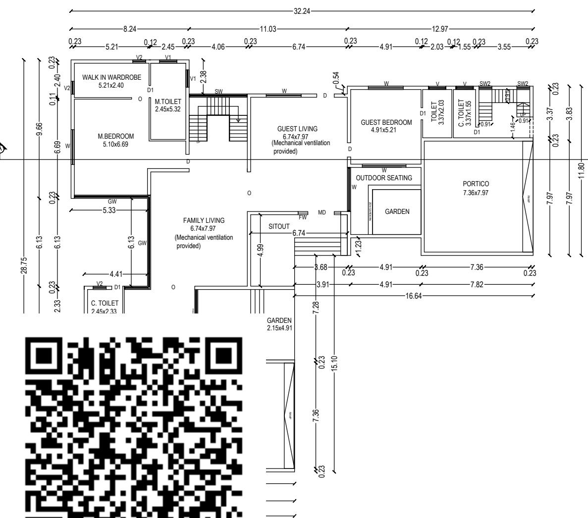
FLOOR PLAN
