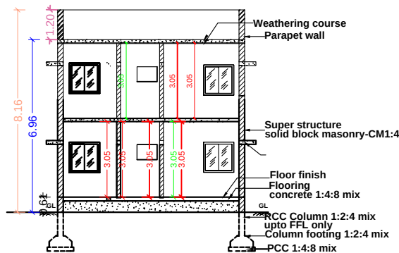
SECTION ELEVATION
