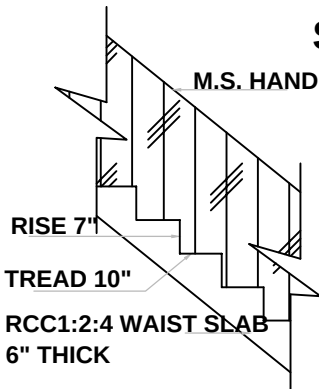
STAIRCASE DETAILS SCALE- 1:20
