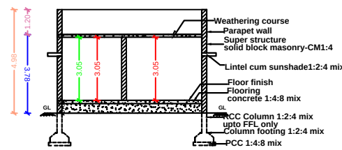
SECTION ELEVATION
