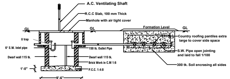
SEPTIC TANK WITH DISPERSION TRENCH ( 250 Gls.,)
