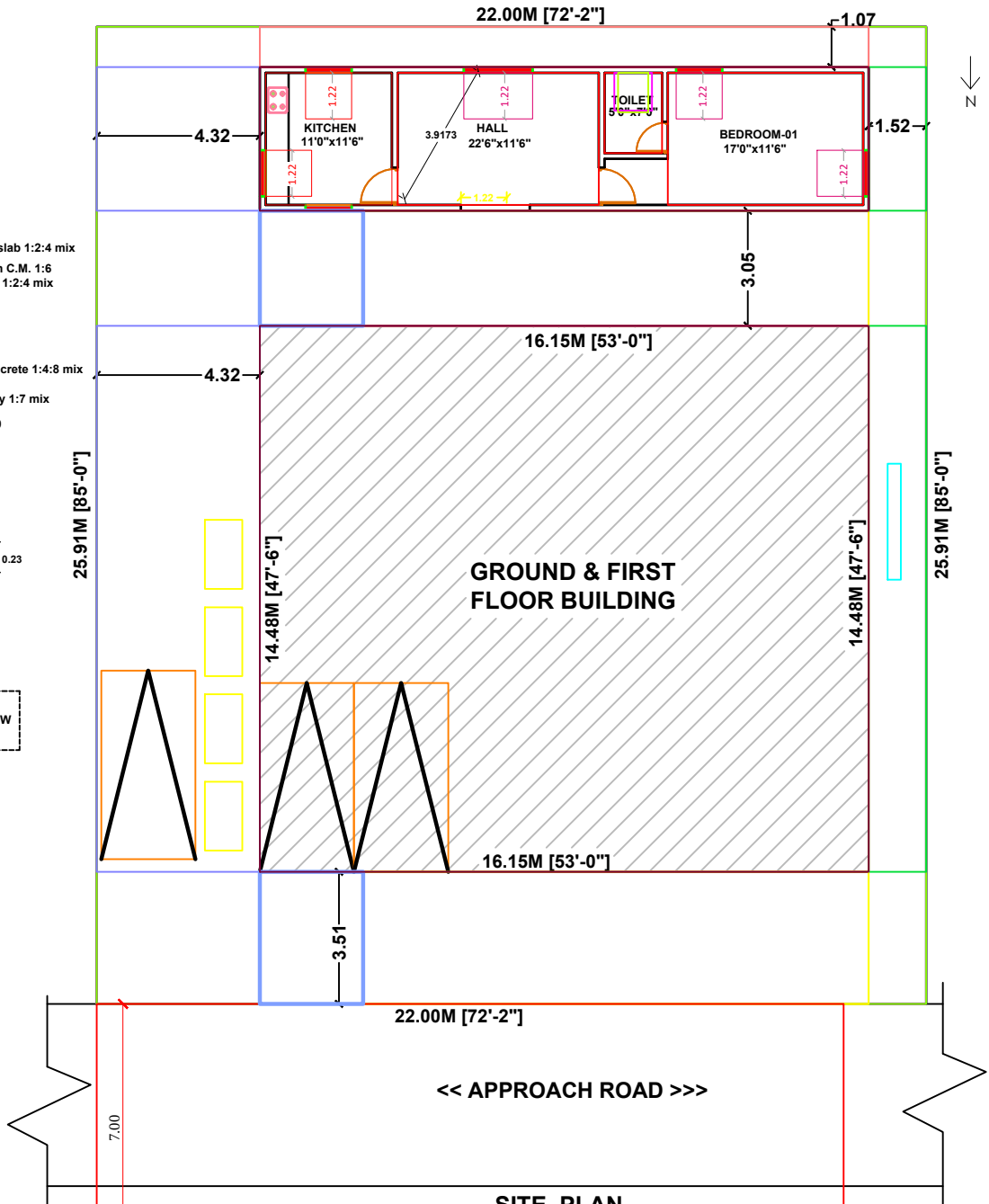
SITE PLAN
