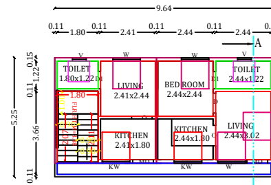
PRO.F.FLOOR PLAN
