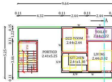
PRO.G.FLOOR PLAN
