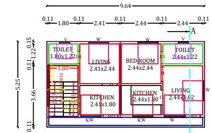
PRO.S.FLOOR PLAN
