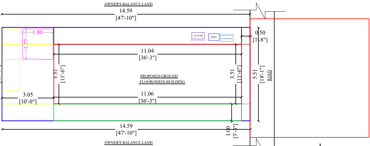
SITE PLAN
