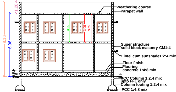
SECTION ELEVATION
