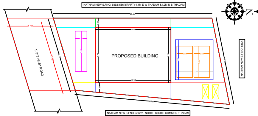
SITE PLAN
