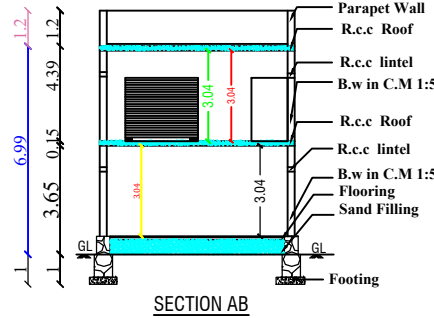
SECTION AB
