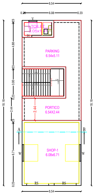
PRO.G.FLOOR PLAN
