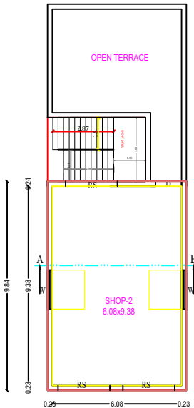
PRO.F.FLOOR PLAN
