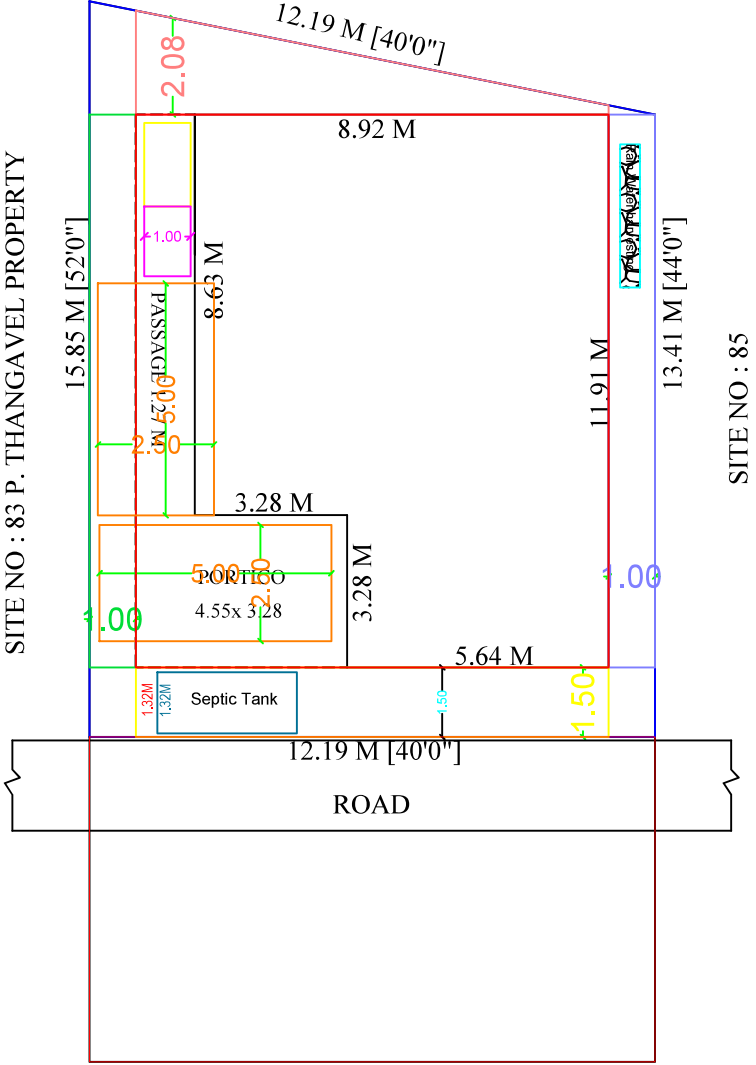
SITE PLAN
