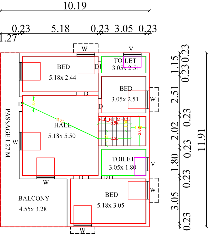
PLAN FOR FIRST FLOOR
