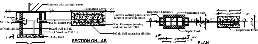
PLAN
