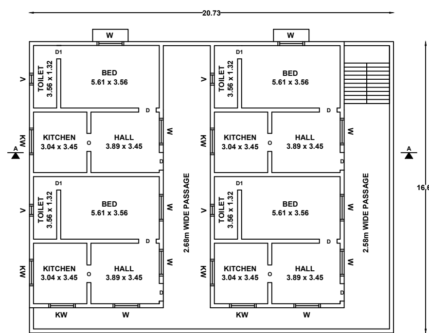
PROPOSED SECOND FLOOR PLAN SCALE - 1' 0\"/>
