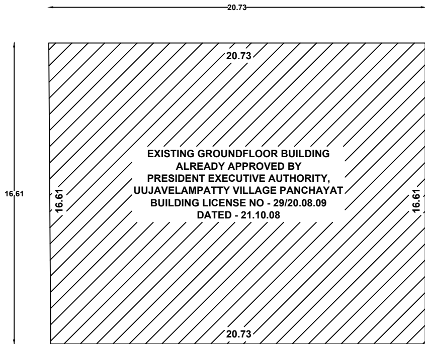
EXISTING GROUND FLOOR PLAN SCALE - 1' 0\"/>
