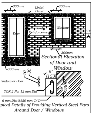
Typical Details of Providing Vertical Steel Bars Around Door / Windows
