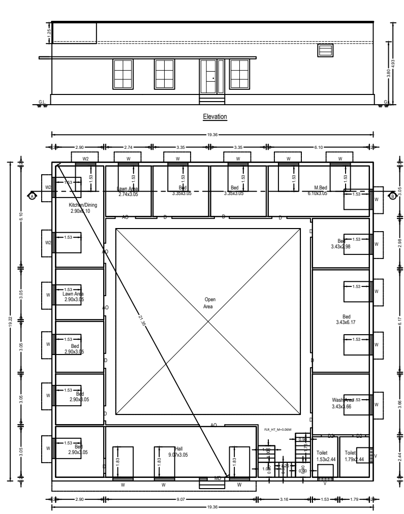
Plan Scale 1:100 Ground floor
