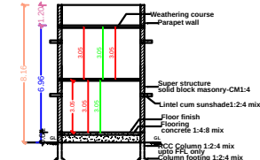
SECTION ELEVATION
