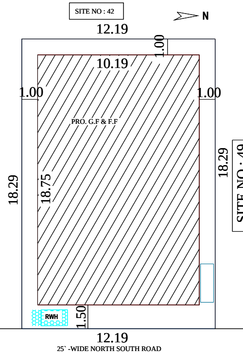
SITE PLAN
