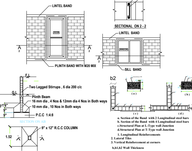
a. Section of the Band with 2 Longitudinal steel bars b. Section of the Band with 4 Longitudinal steel bars c. Structural Plan at L-Type wall Junction d. Structural Plan at T-Type wall Junction 1. Longitudinal Reinforcements 2. Lateral Ties 3. Vertical Reinforcement at corners b.b.l.b2 Wall Thickness
