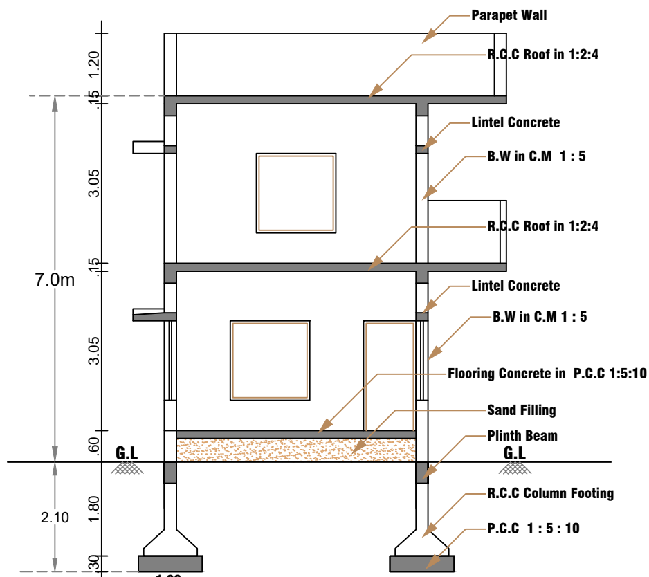
SECTION THROUGH "AA"
