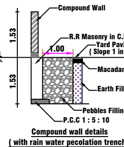
Compound wall details (with rain water percolation trench)
