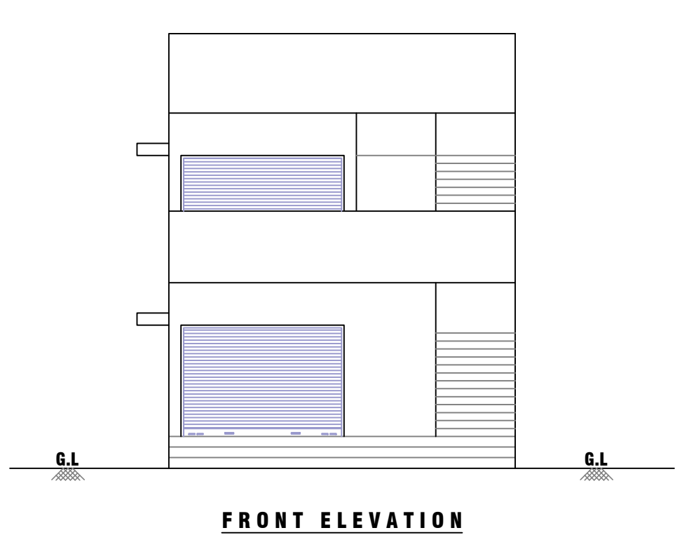
FRONT ELEVATION
