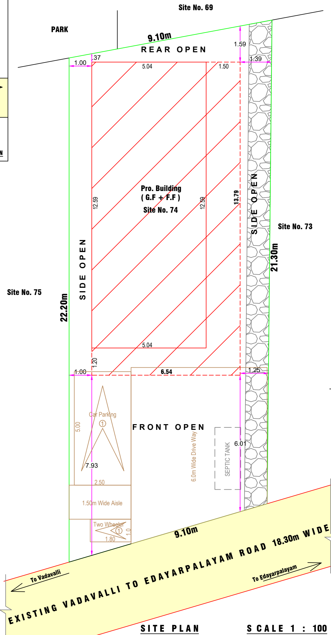
SITE PLAN
