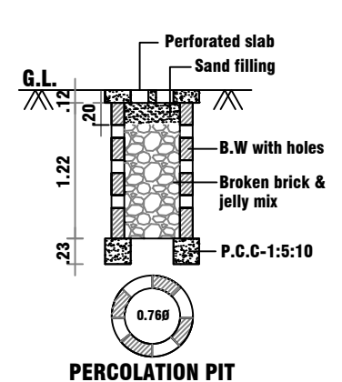
PERCOLATION PIT
