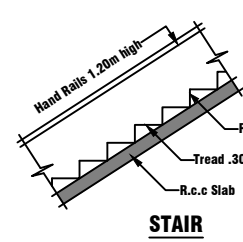
STAIR
