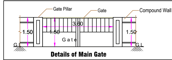
Details of Main Gate
