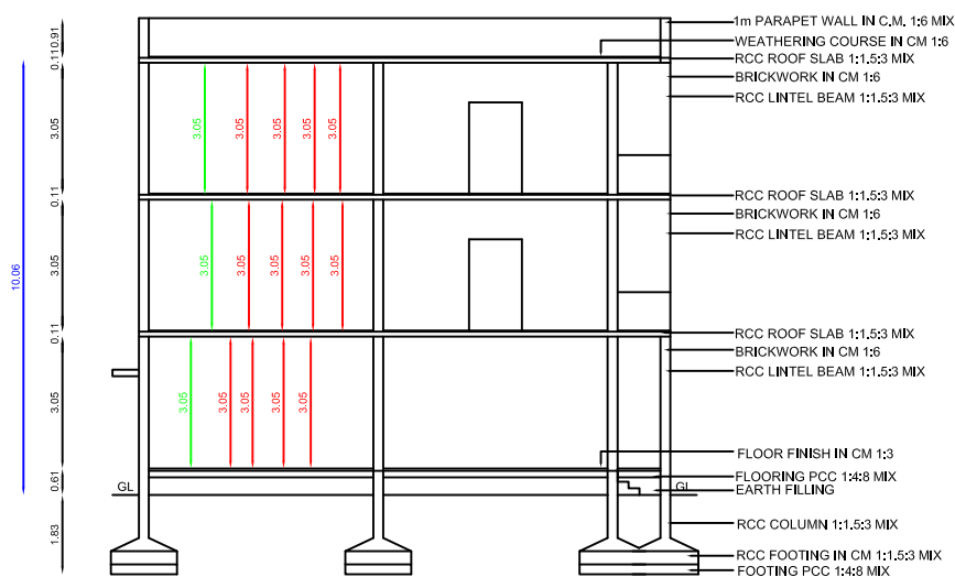
CROSS SECTION ON XY
