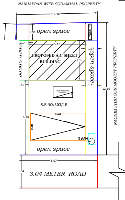
SITE PLAN
