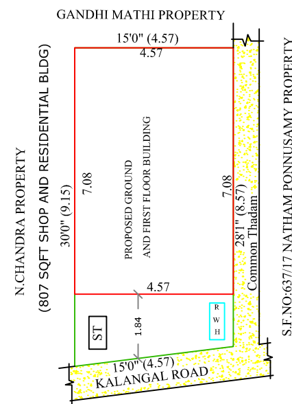
SITE PLAN
