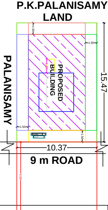
SITE PLAN
