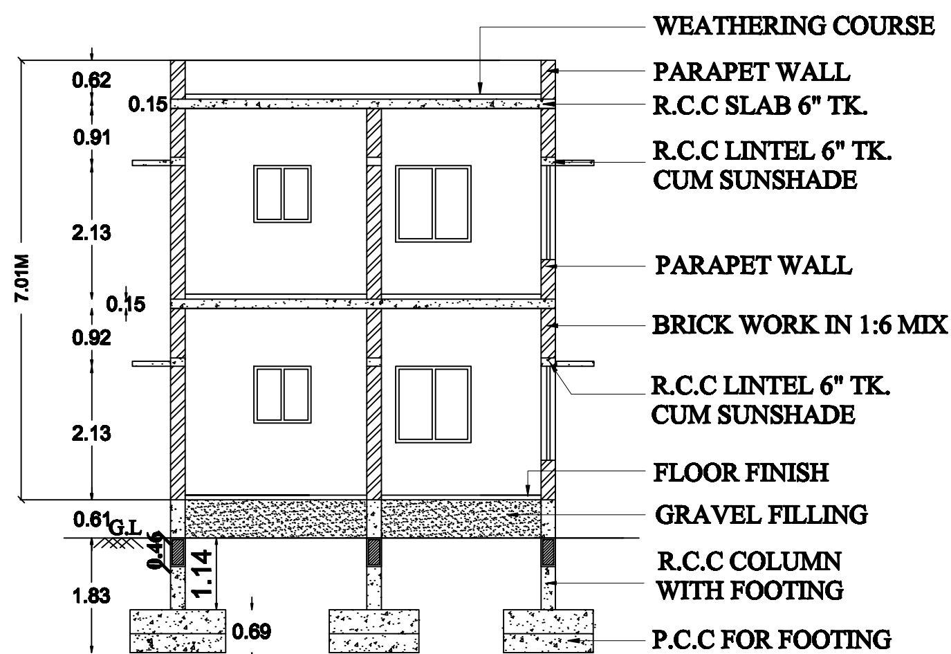
CROSS SECTION AT A-A
