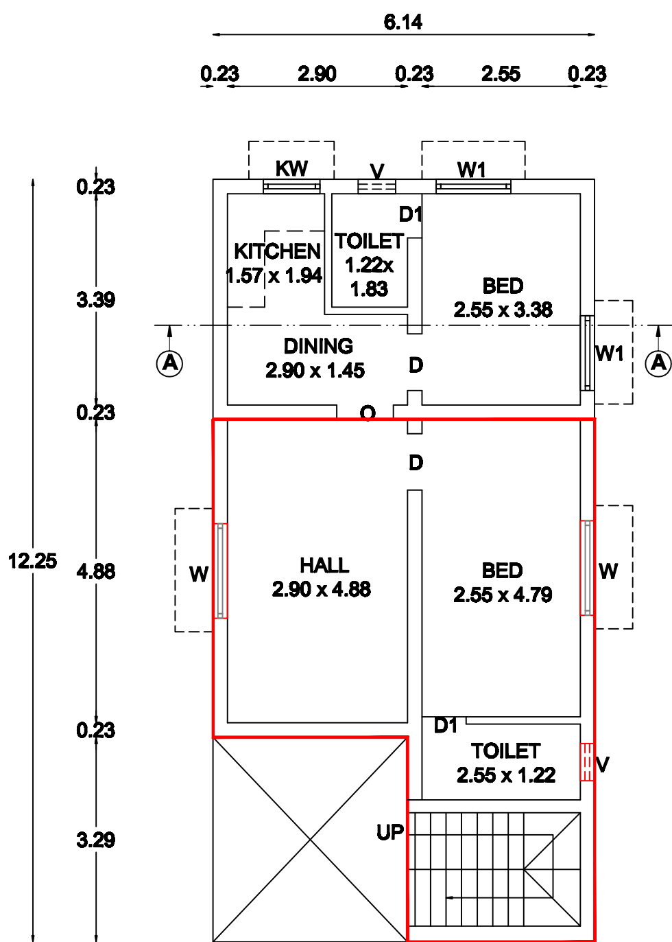
EXISTING FIRST FLOOR & PROPOSED FIRST FLOOR PLAN
