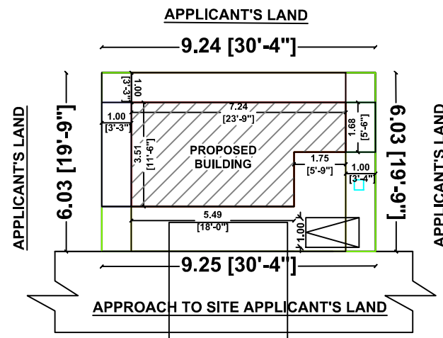
SUPER IMPOSED SITE PLAN
