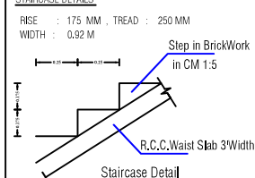
STAIRCASE DETAILS
