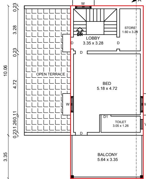
PRO. ADDL. FIRST FLOOR PLAN
