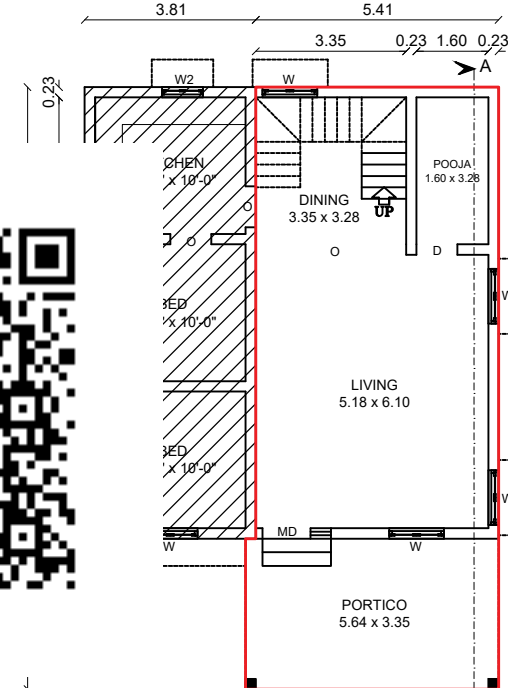
EXI. PRO. ADDL. GROUND FLOOR PLAN
