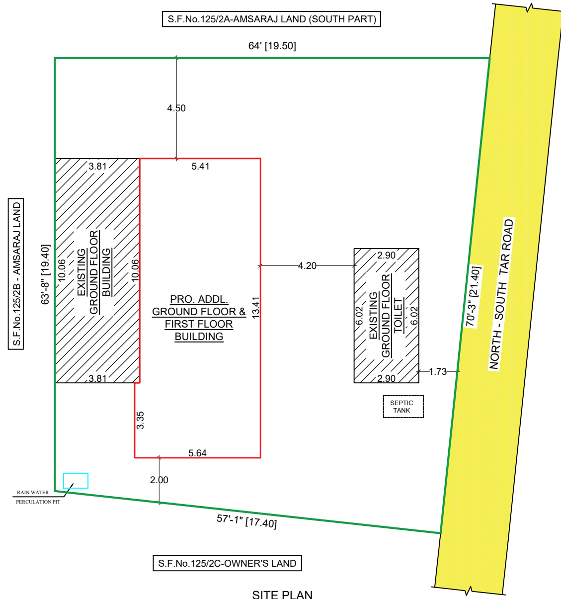
SITE PLAN
