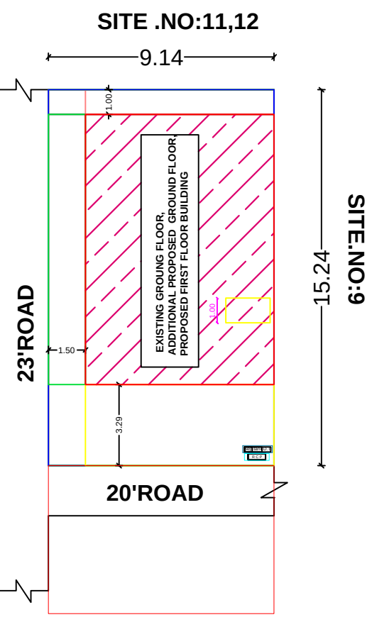
SITE PLAN
