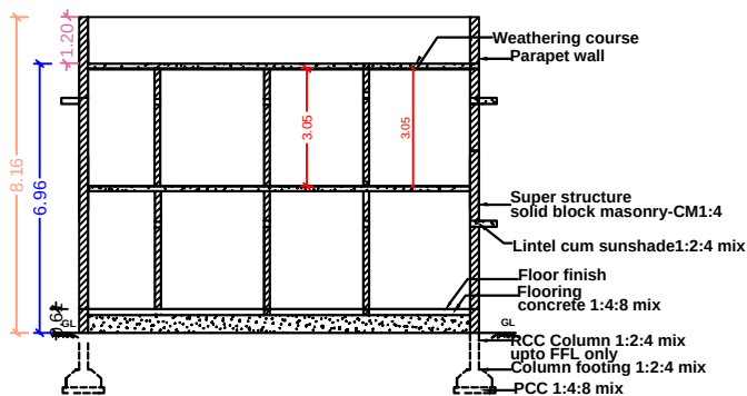
SECTION ELEVATION
