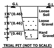
TRIAL PIT (NOT TO SCALE)
