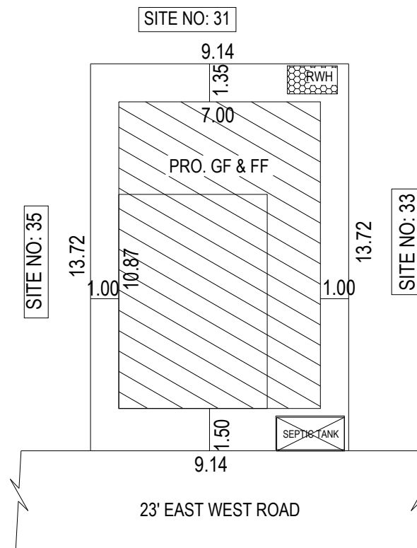
SITE PLAN
