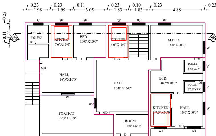
ADDITION & ALTERATION OF GROUND FLOOR PLAN
