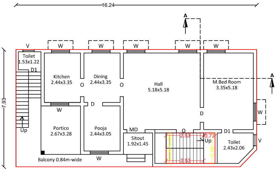
EXI GF PLAN
