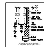
COMPOUND WALL
