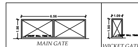
WICKET GATE
