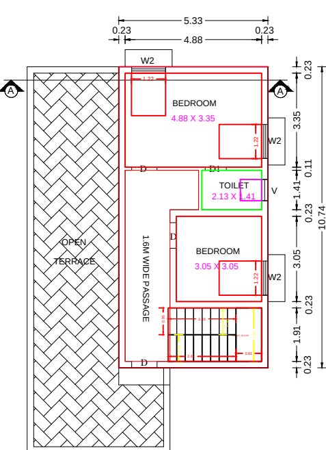
PRO. SECOND FLOOR PLAN
